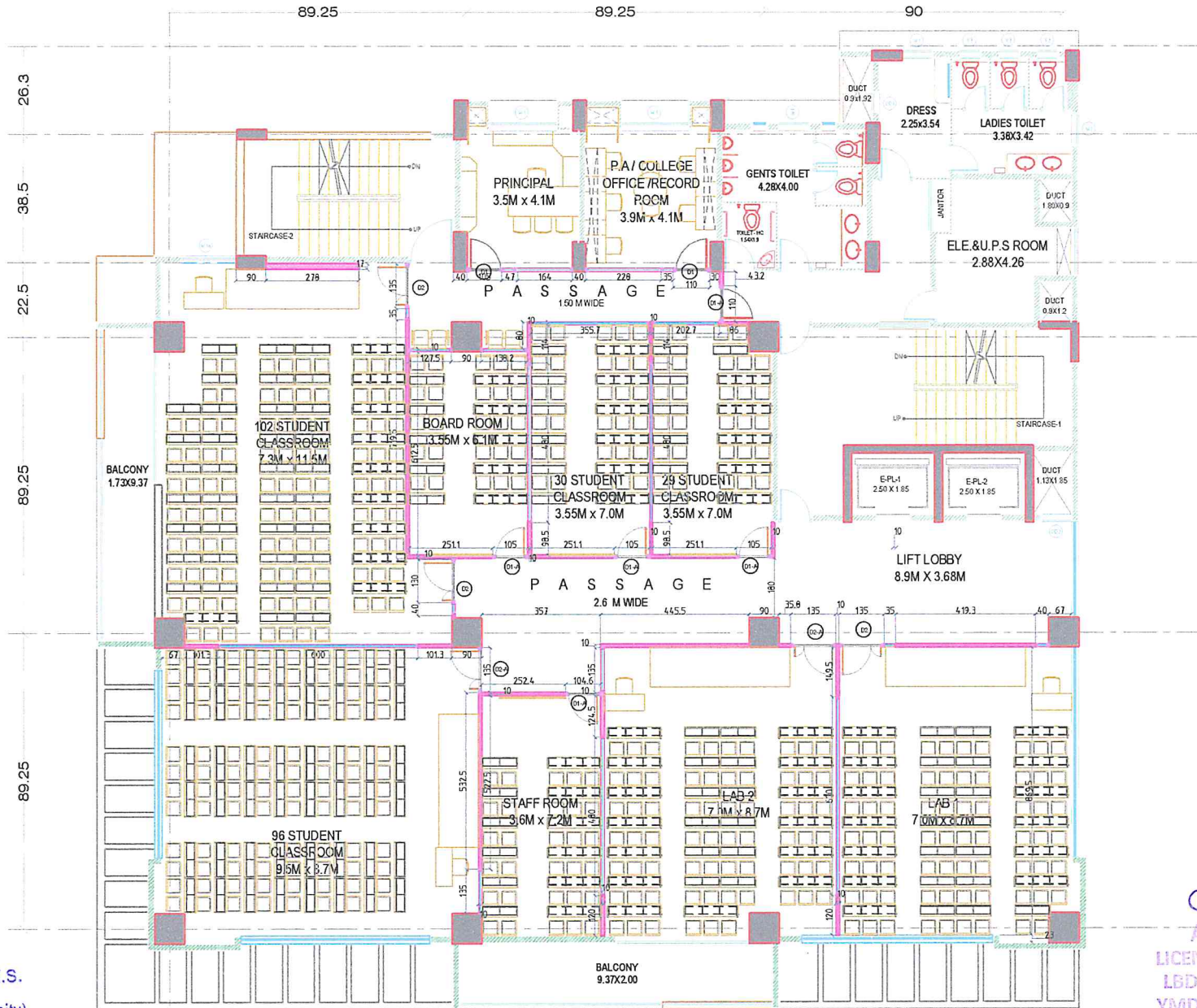
2 FLOOR PLAN Page: 60 of 100
