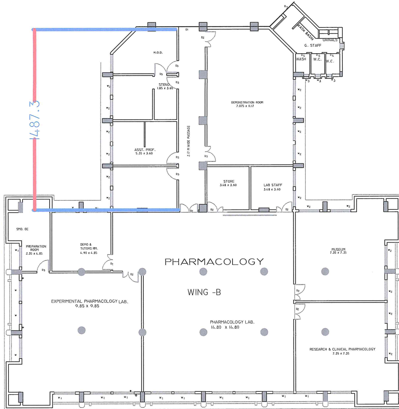
WING -B FIRST FLOOR PLAN
